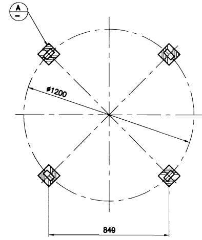
FOUNDATION
