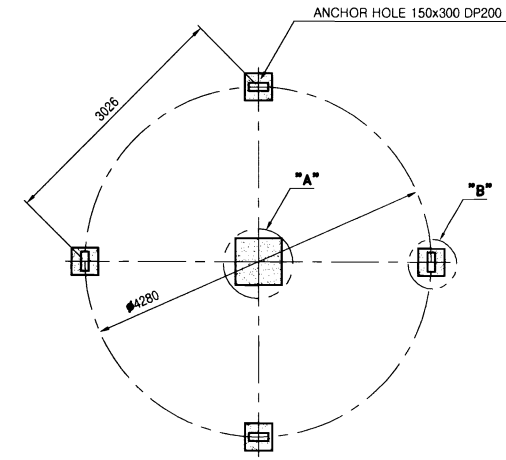
BASE FOUNDATION
