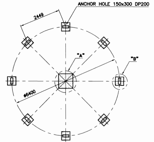
BASE FOUNDATION
