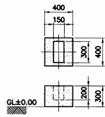
DETAIL "B"
