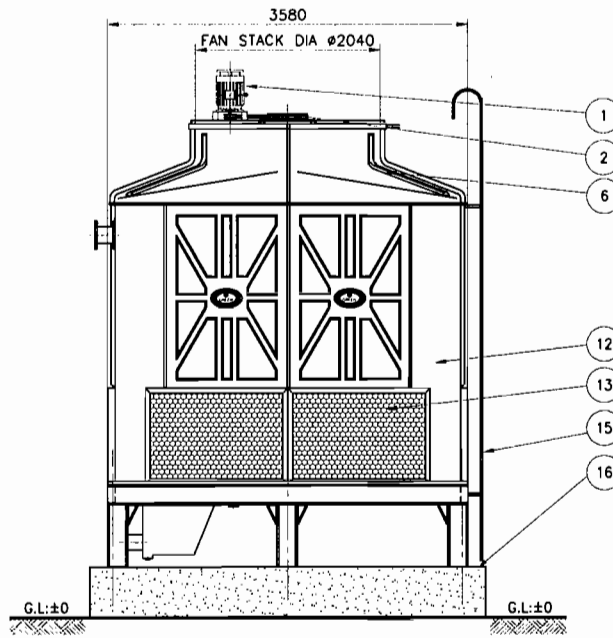
Concrete Foundation
