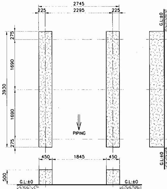
Concrete Foundation
