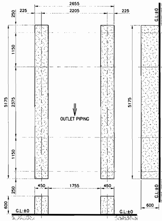
Concrete Foundation
