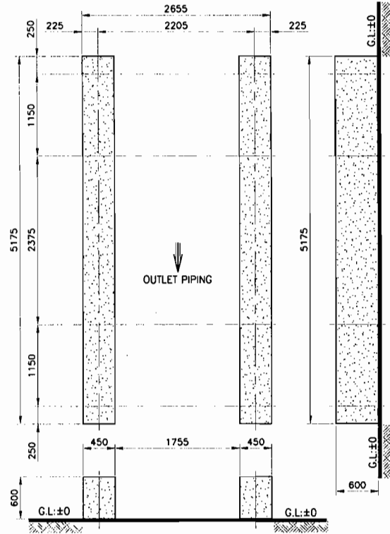
Concrete Foundation
