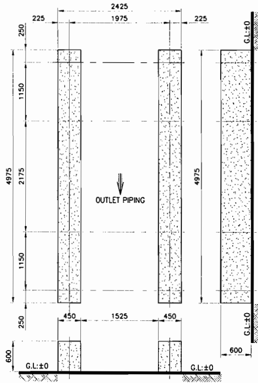
Concrete Foundation
